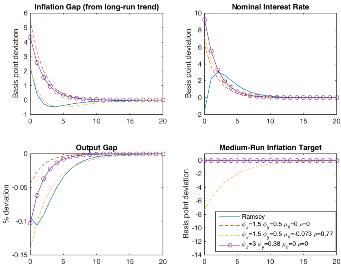
Figure 3: Impulse response to a 1% cost-push shock
