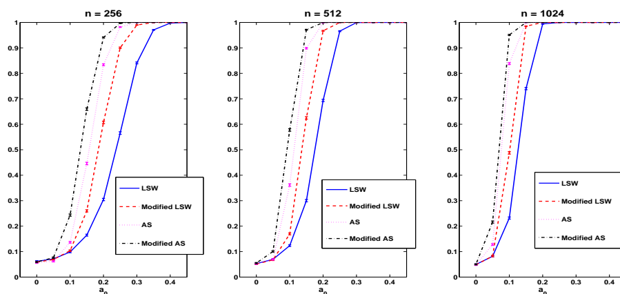
Fig. 8. The empirical rejection probabilities under the alternative: directions of non-dominance.
