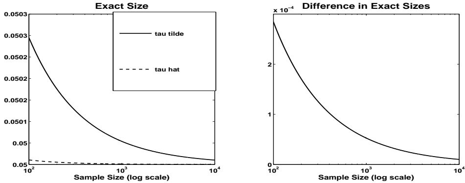
Fig. 3. The first panel reports the exact sizes of the tests \hat{\tau}_n and \tilde{\tau}_n . The second panel reports the difference \sup_{P \in \mathcal{M}_0} E_P \hat{\tau}_n - \sup_{P \in \mathcal{M}_0} E_P \tilde{\tau}_n .
