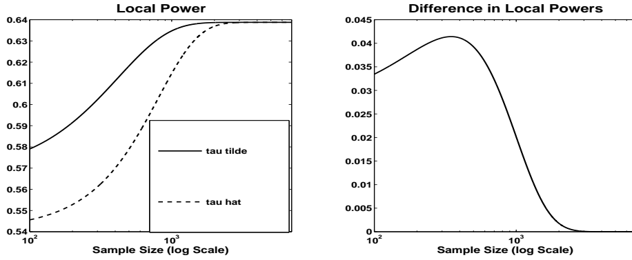
Fig. 4. The left panel plots the local powers E_{P_n} \hat{\tau}_n and E_{P_n} \tilde{\tau}_n . The right panel plots the difference E_{P_n} \tilde{\tau}_n - E_{P_n} \hat{\tau}_n .
