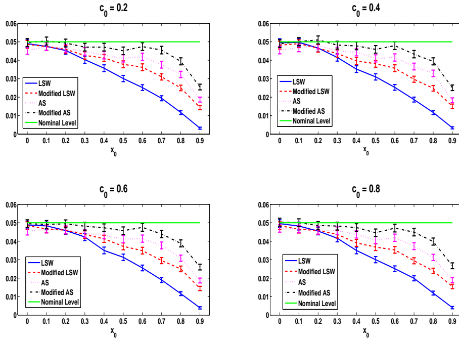
Fig. 7. The empirical rejection probabilities under the null.
