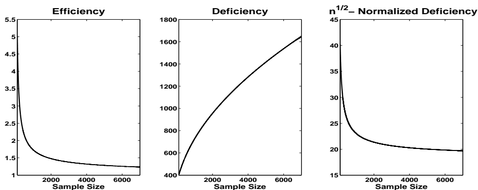
Fig. 5. The panels, from left to right, plot the efficiency k_n/n , deficiency d_n , and normalized deficiency d_n/\sqrt{n} of \hat{\tau}_n with respect to \tilde{\tau}_n , respectively.
