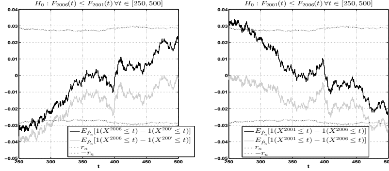
Fig. 2. The left panel reports E_{\hat{P}_n}[g(\mathbf{X}, \cdot)] and E_{\hat{P}_n}[g(\mathbf{X}, \cdot)] , and the values of the localization parameter r_n(\cdot) for the test problem (6.1). The right panel reports the same quantities but for the test problem (6.2).
