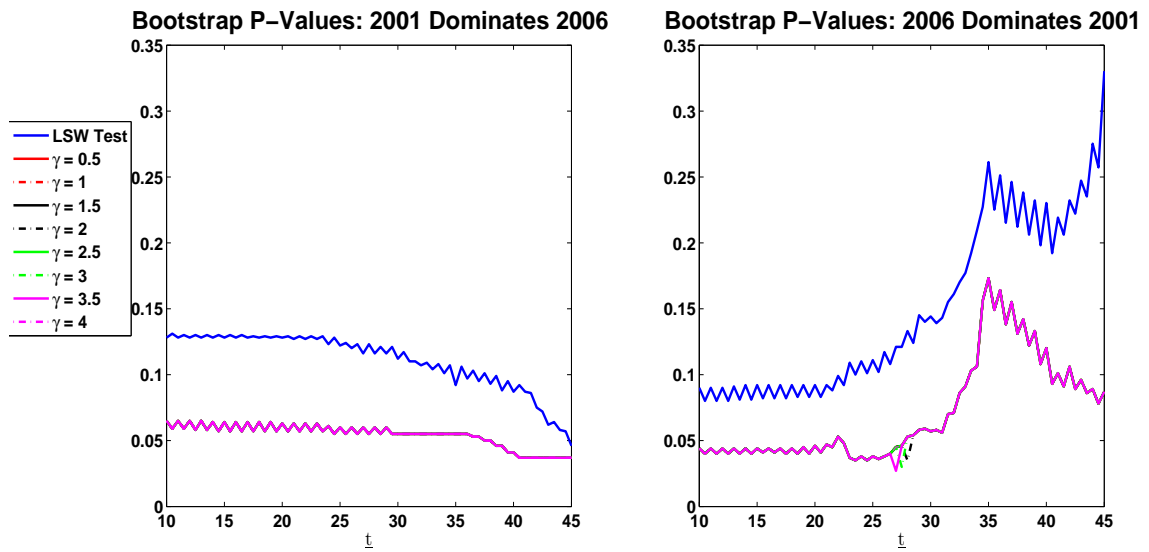
Figure 5: Bootstrap P-Values
